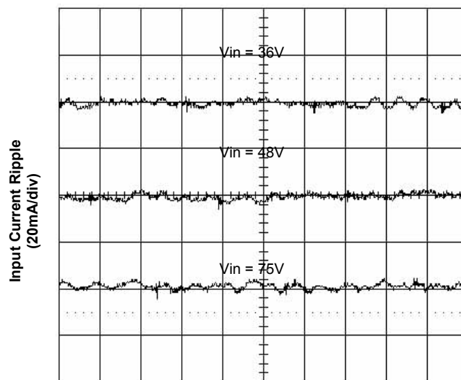
Figure 6. Input Reflected Ripple Current at 10A Load
