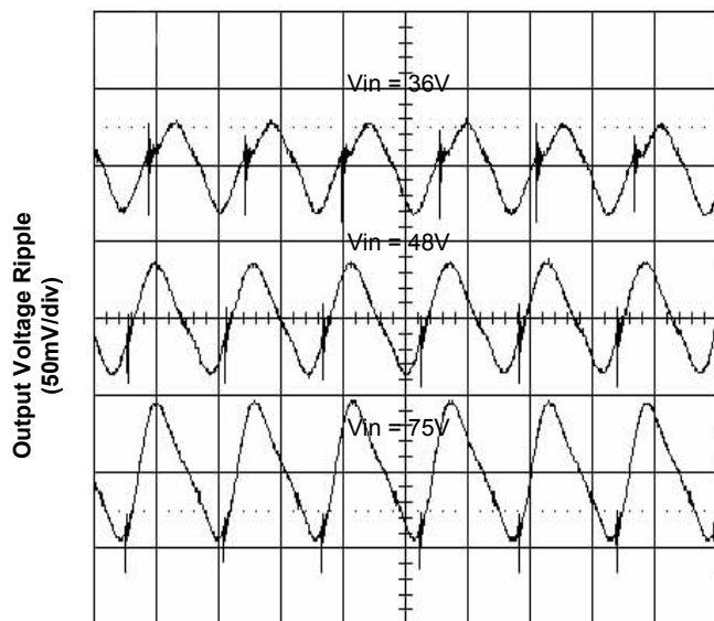
Figure 5. Output Ripple Voltage at 10A Load
