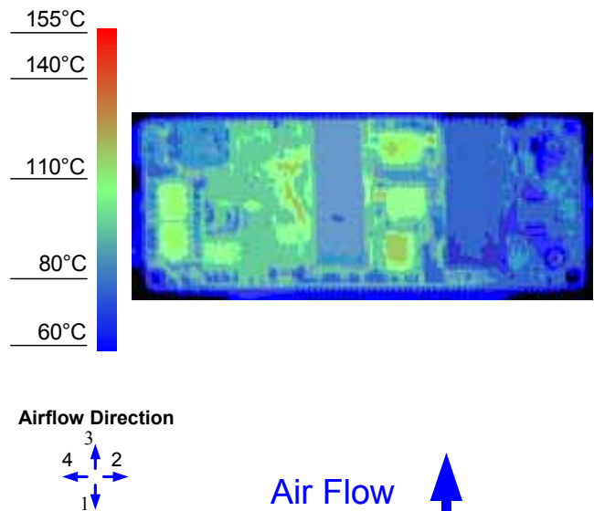
Figure 12. Thermal Image for Airflow Direction 3 (8.8A output, 55°C ambient, 200 LFM, V_{in} = 48V open frame unit using socket interface)
