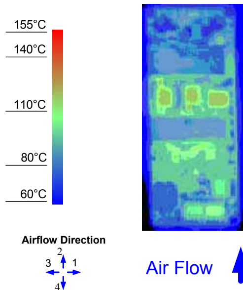
Figure 14. Thermal Image for Airflow Direction 2 (7.5A output, 55°C ambient, 200 LFM, Vin = 48V open frame unit using solder interface)
