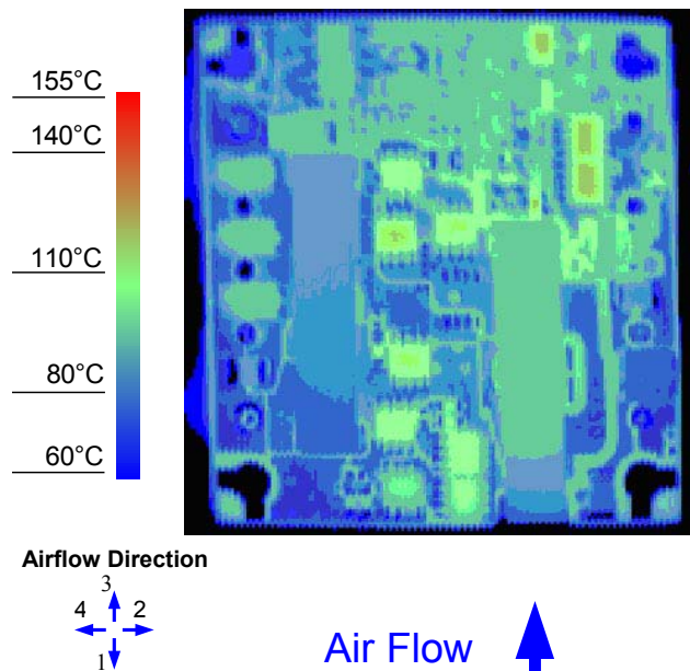
Figure 12. Thermal Image for Airflow Direction 3 (36.5A output, 25°C ambient, 200 LFM, Vin = 48V open frame unit using socket interface)
