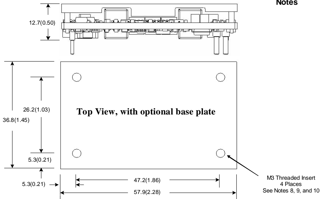
Figure 24. Converter with a baseplate
