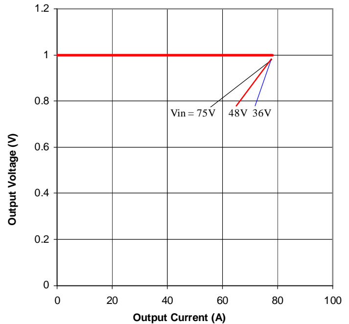
Figure 10. Output Characteristics
