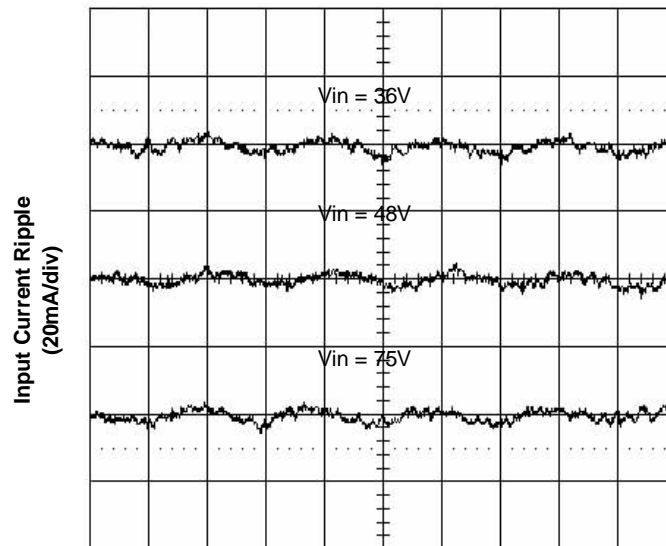
Figure 6. Input Reflected Ripple Current at 70A Load
