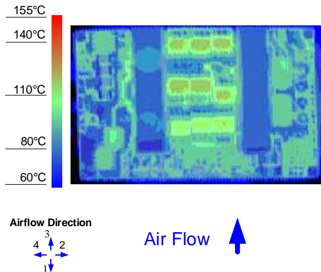
Figure 12. Thermal Image for Airflow Direction 3 (58.5A output, 55 ^{\circ}C ambient, 200 LFM, V_{in} = 48V open frame unit using socket interface)
