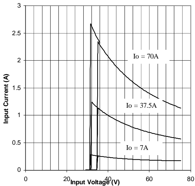
Figure 9. Input Characteristics
