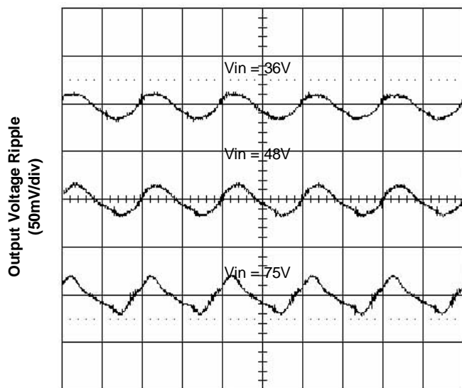
Figure 5. Output Ripple Voltage at 70A Load
