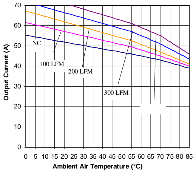
Figure 13. Current Derating Curve for Airflow Direction 2 (Ref. Fig.14 for Airflow Direction; Vin = 48V open frame unit using socket interface)
