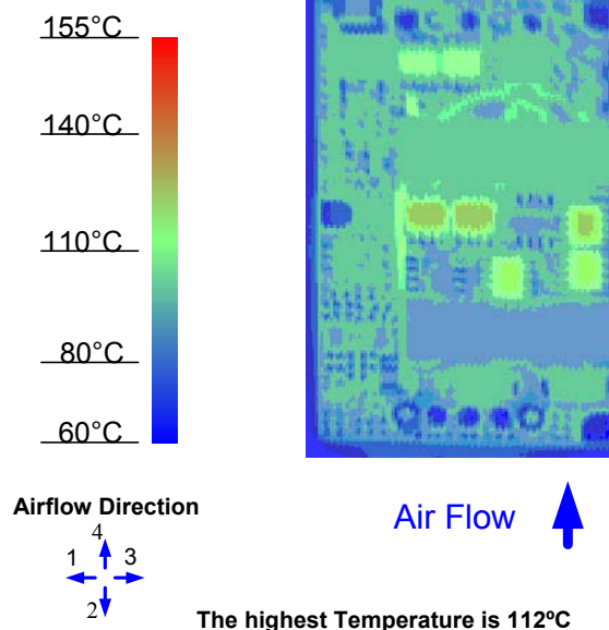
Figure 14. Thermal Image for Airflow Direction 4 (28A output, 55°C ambient, 200 LFM, Vin = 48V open frame unit using solder interface)
