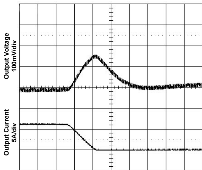
Time - t (50μs/div) Figure 7. Transient Load Response
