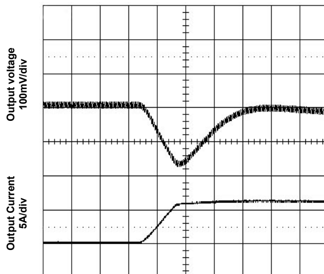
Time - t (50μs/div) Figure 8. Transient Load Response
