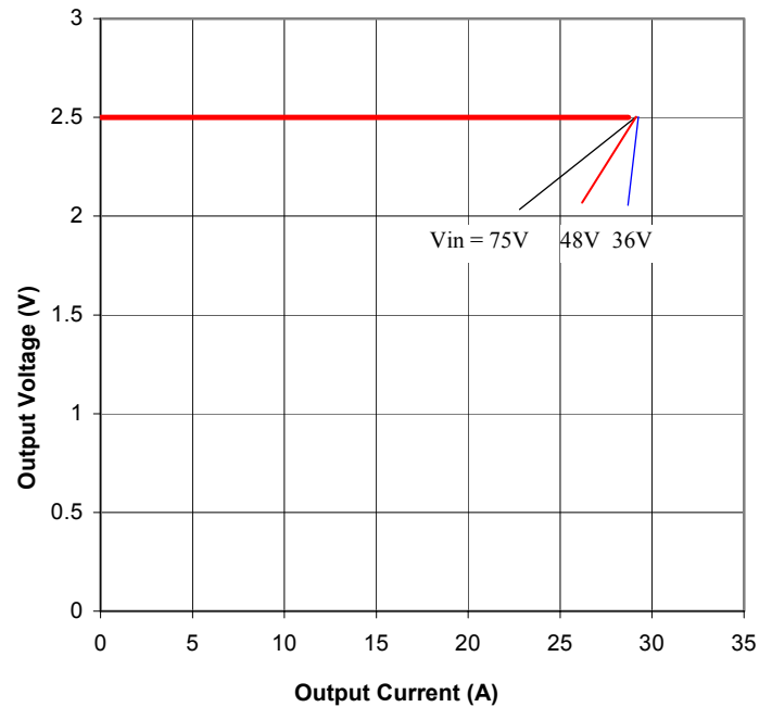
Figure 10. Output Characteristics
