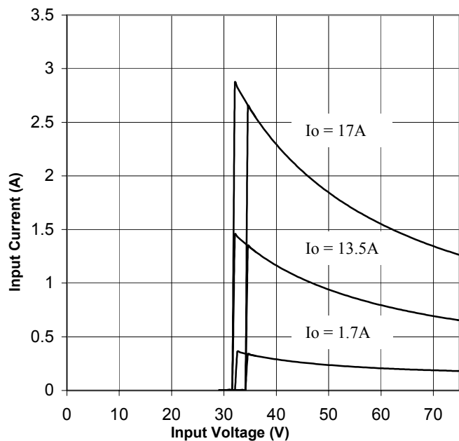
Figure 9. Input Characteristics
