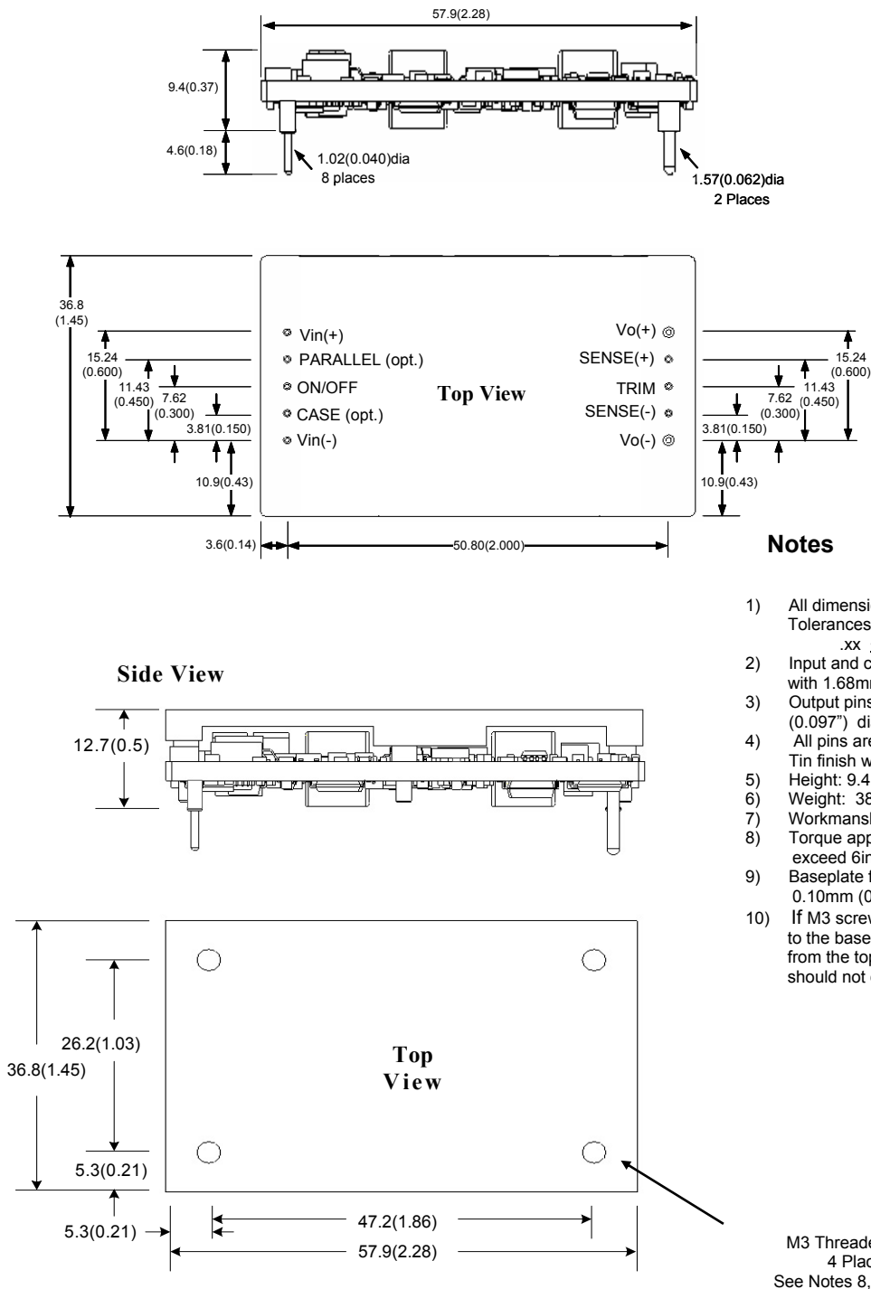
Figure 25. Converter with Optional Baseplate
