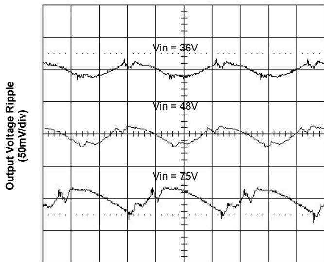
Figure 5. Output Ripple Voltage at 17A Load
