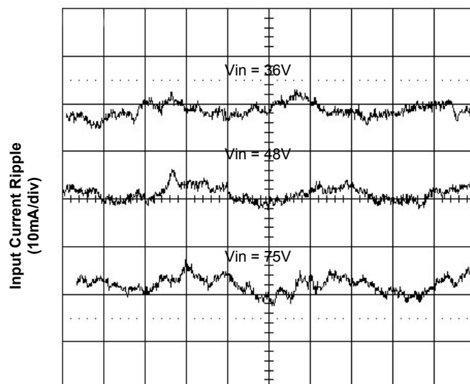
Figure 6. Input Reflected Ripple Current at 17A Load
