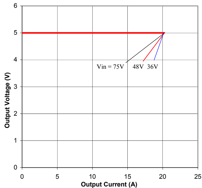
Figure 10. Output Characteristics
