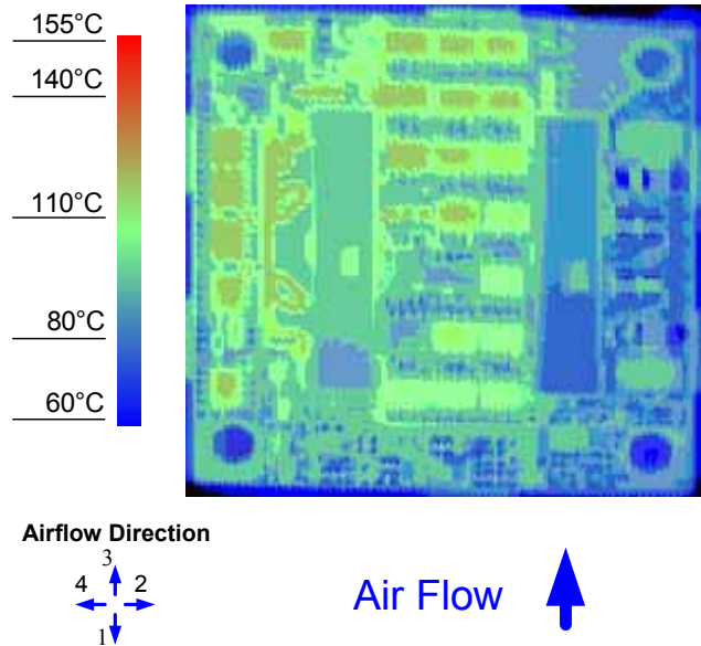
Figure 12. Thermal Image for Airflow Direction 3 (34A output, 55°C ambient, 200 LFM, V_{in} = 48V open frame unit using socket interface)
