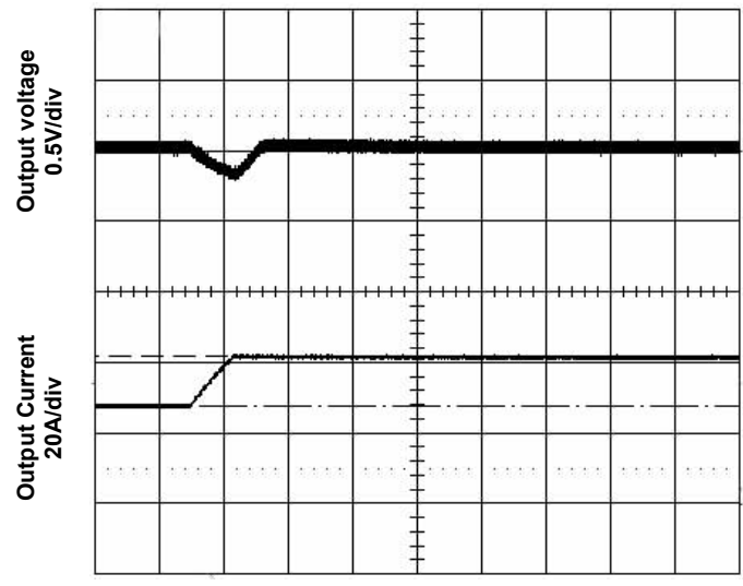
Time - t (200µs/div) Figure 8. Transient Load Response
