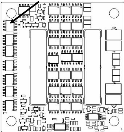
Figure 23. Temperature Monitoring Location
