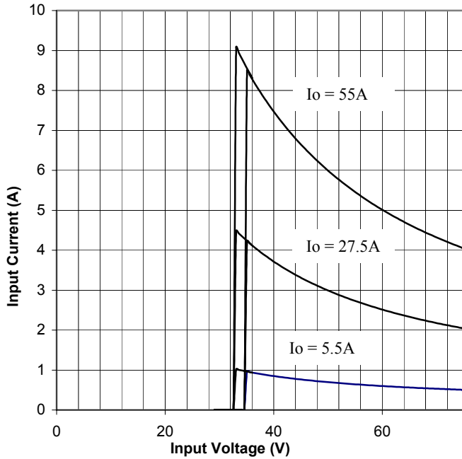
Figure 9. Input Characteristics
