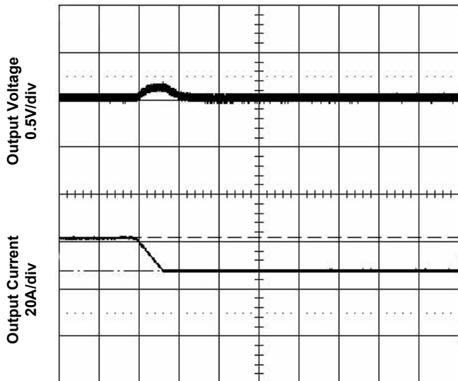
Time - t (200µs/div) Figure 7. Transient Load Response
