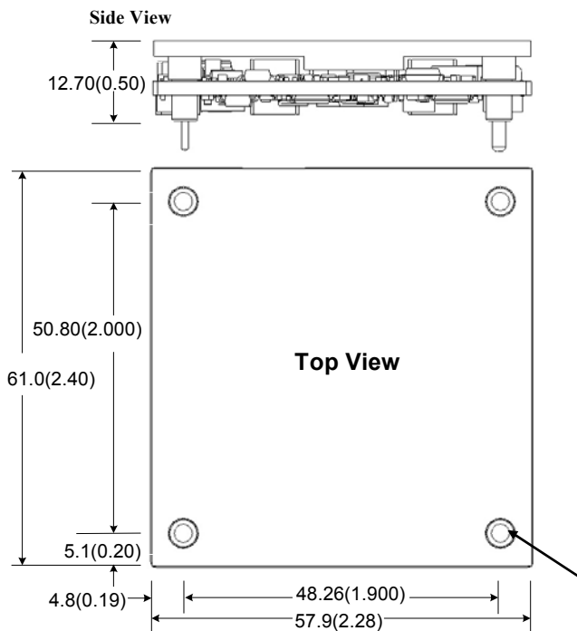
Figure 25. Converter with Optional Baseplate
