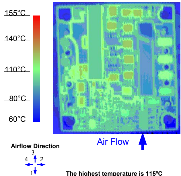
Figure 12. Thermal Image for Airflow Direction 1 (40A output, 70 ^{\circ}C ambient, 200 LFM, V_{in} = 48V open frame unit using socket interface)
