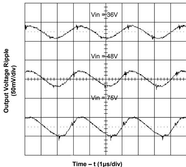
Figure 5. Output Ripple Voltage at 40A Load
