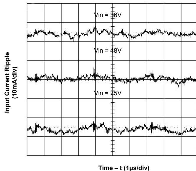
Figure 6. Input Reflected Ripple Current at 40A Load
