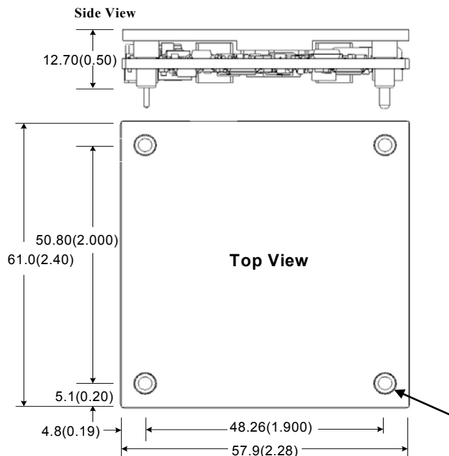
Figure 25. Converter with Optional Baseplate
