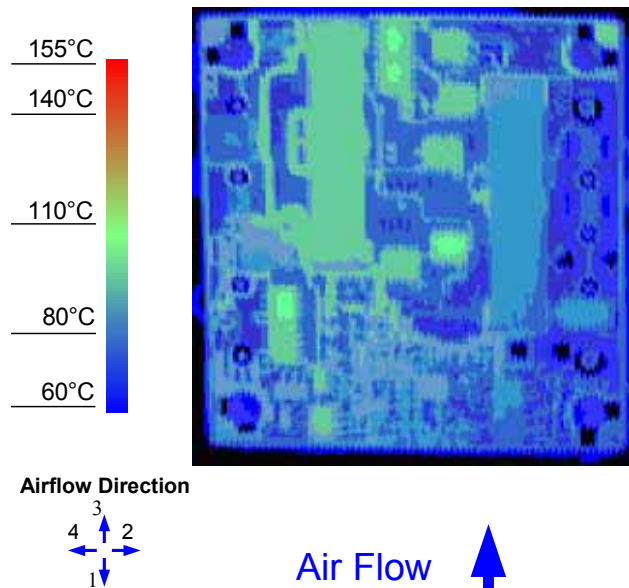
Figure 12. Thermal Image for Airflow Direction 3 (25A output, 55°C ambient, 200 LFM, Vin = 48V open frame unit using socket interface)
